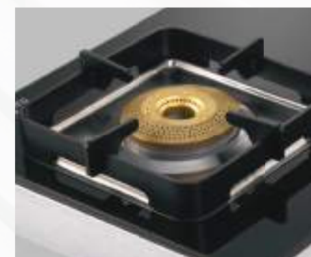
Strong Fuel Efficient Pan Support provides sturdy support for stable, spill-free cooking.
